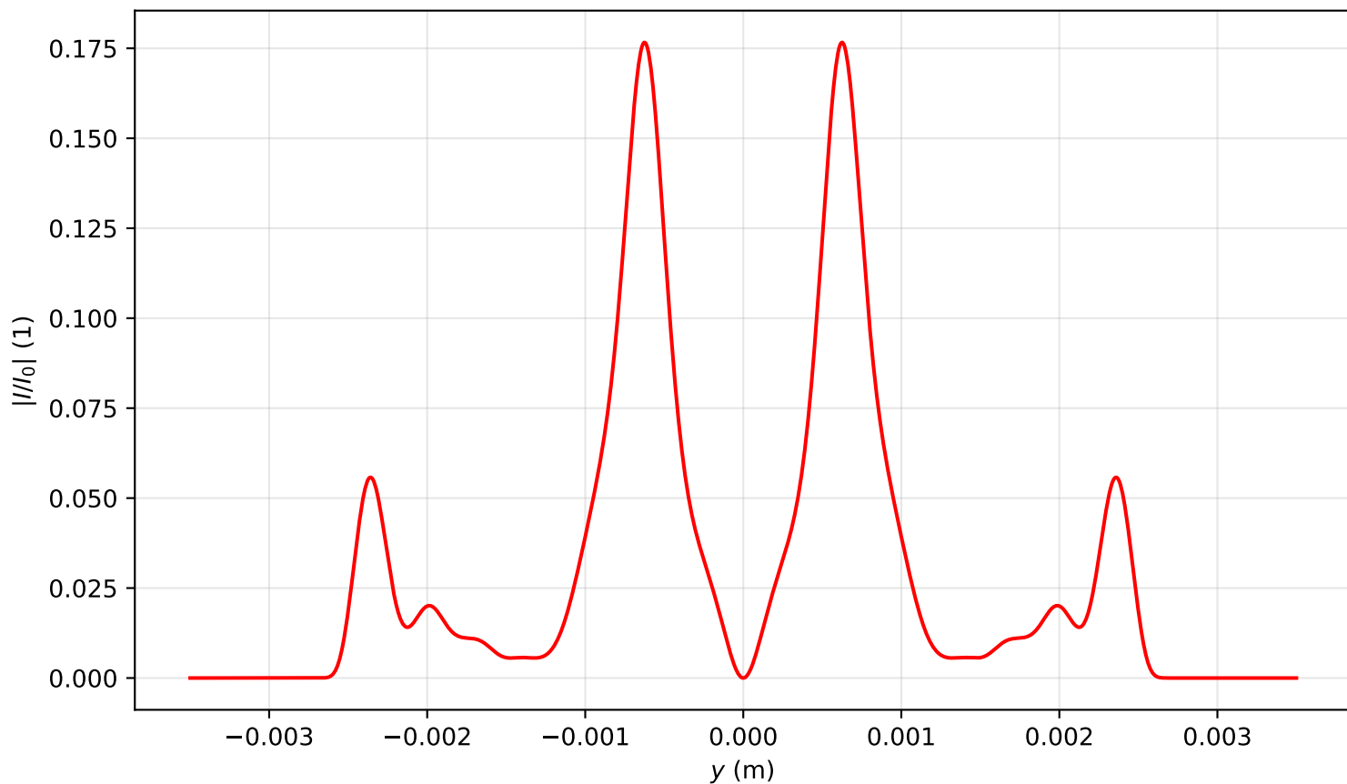
Intensity profile I(x=0, y, z=3.662)/I_0 , Pin=9.0Pcr, artificial time
